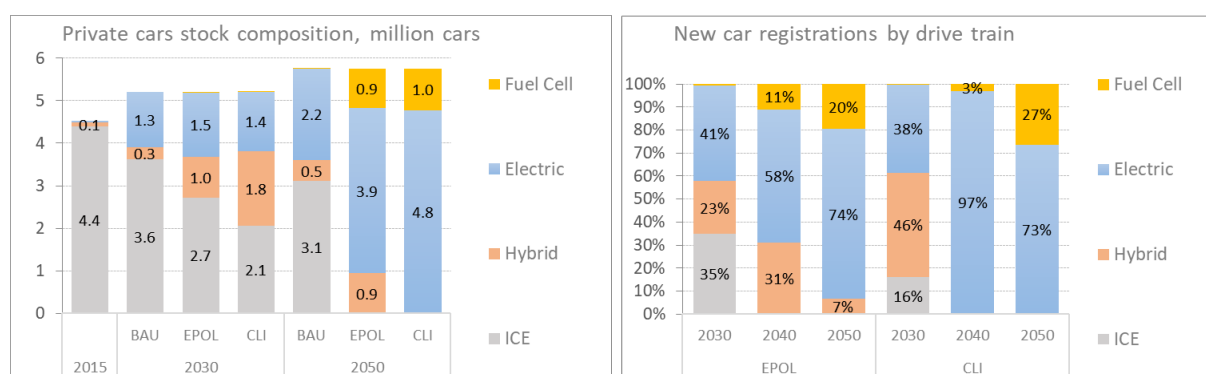
Figure 3.16: Composition of private car fleet (left), and share of drive trains in new private car registrations. ICE refers to Internal Combustion Engine vehicles fuelled by gasoline, diesel, natural gas and biofuels. Electric refers to both plugin and battery electric vehicles where plugins can be fuelled by gasoline, diesel, biofuels and synfuels. Fuel cell electric vehicles are based on hydrogen
