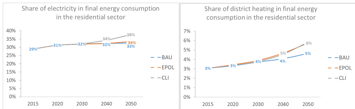
Figure 3.6: Share of electricity (left) and consumption of district heating (right) in the residential sector
