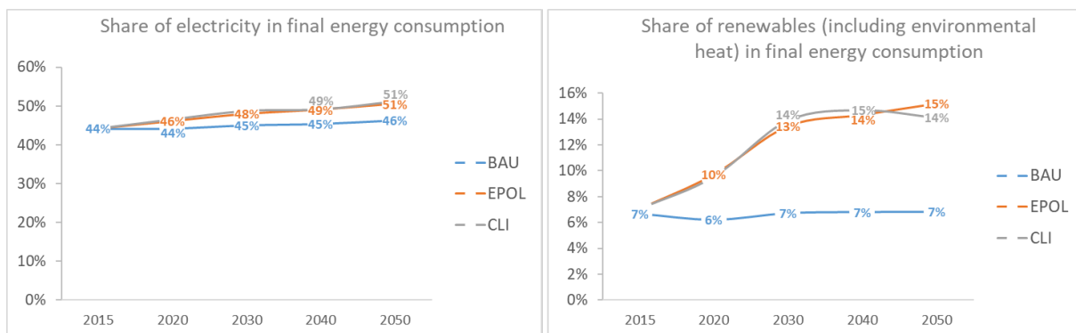
Figure 3.10: Share of electricity (left) and share of renewable energy (right) in the total final energy consumption in industry
